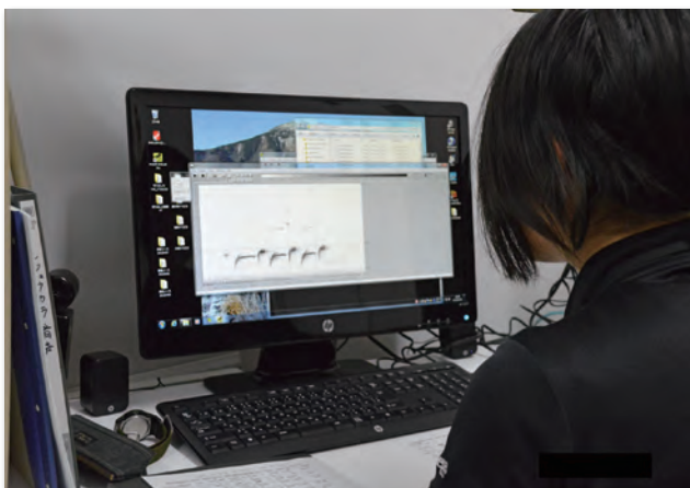
鳥類の音声の分析 Acoustic analysis of an avian vocalization
