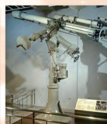
(右下)観測に使われた20cm屈折赤道儀 (Lower Right) 20cm refracting telescope used for observation
