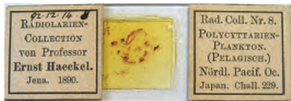
Fig. 3. Haeckel radiolarian teaching slide, No. 8, North Pacific Ocean, Japan Challenger Station 229, Reg. No. 92.12.14.8
