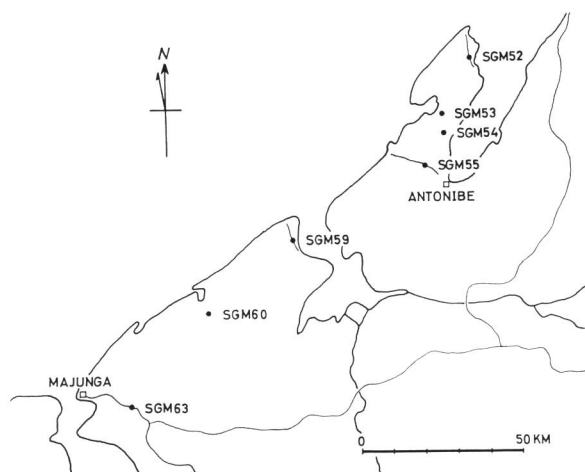
Fig. 2. Localities of the Danian Hercoglossa near Antonibe and Majunga, adapted from BESAIRES, 1976. SGM means the locality number of the Service Géologique of Madagascar.
