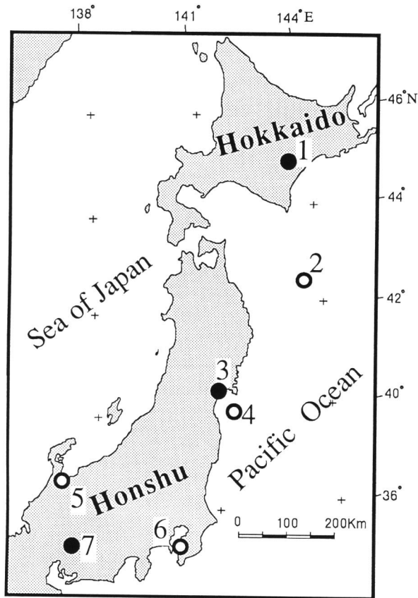
Fig. 1. Locality of selected Cenozoic sequences in Japan treated in this paper. Black circles indicate type localities of new taxa of Cavitatus . 1, The Tokiwa Formation and the Okubonosawa Section: Holotype locality of Cavitatus rectus sp. nov. 2, DSDP, Leg 57, Site 438A. 3, The Otsuka Formation, Matsushima area, Miyagi Prefecture: Holotype locality of Cavitatus lanceolatus sp. nov. 4, An offshore well, MITI-Souma-oki. 5, Neogene sequences in Kanazawa area, Ishikawa Prefecture and Yatsuo area, Toyama Prefecture. 6, The Okuyama Formation of the Sakuma Group, Boso Peninsula, Chiba Prefecture. 7, The Oidawara Formation, Mizunami area, Gifu Prefecture: Holotype locality of Cavitatus exiguus sp. nov.
