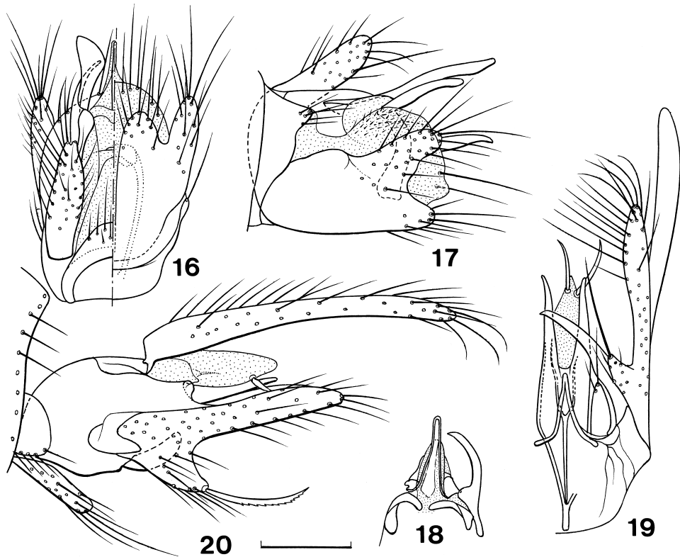
Figs. 16–20. Male genitalia of Epicypota dolabrata n. sp. (holotype, 16–18) and Epicypota longistylis n. sp. (paratype, 19–20). 17, 20, Gonocoxite and gonostylus, lateral view; 18, aedeagus, ventral view; 19, gonostylus and aedeagus, ventral view. Scale 0.1 mm.
