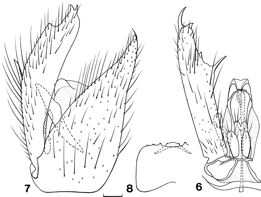
Figs. 6–8. Male genitalia of Allactoneura akasakana n. sp. (paratype). 6, Gonocoxite and aedeagus, dorsal view; 7, gonocoxite and gonostylus, lateral view; 8, half of eighth sternite. Scale 0.1 mm.
