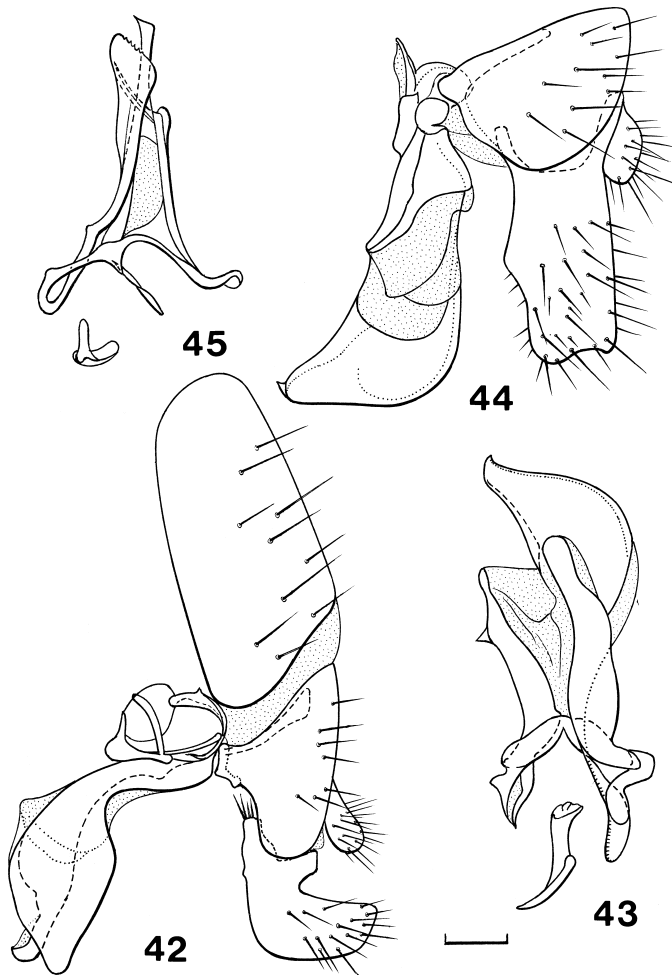
Figs. 42–45. Male genitalia of Itomyia curvata n. sp. (holotype, 42–43) and Itomyia lobata n. sp. (holotype, 44–45). 42, 44, Epandrium, surstylus and aedeagus, lateral view; 43, 45, hypandrium, aedeagus and ejaculatory apodeme, ventral view. Scale 0.1 mm.
