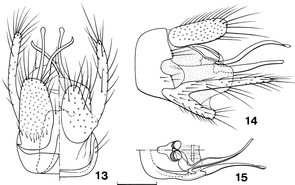
Figs. 13–15. Male genitalia of Epicrypta cruciata n. sp. (paratype). 14, Gonocoxite and gonostylus, lateral view; 15, stylomeres and aedeagus, ventral view. Scale 0.1 mm. See Figs. 1–5.
