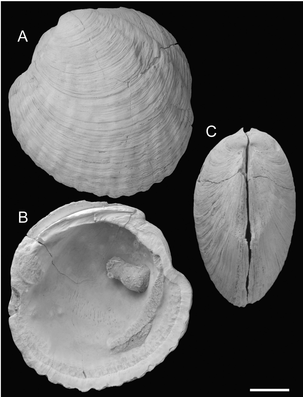
Fig. 3. Paratypes of Bulacanites obtusiplicatus sp. nov. from the same locality of the holotype. A & B, Exterior and interior of left valve, respectively, NSM PM14861; C, anterior view of conjoined valves, NSM PM14862. Scale bar: 20 mm.
