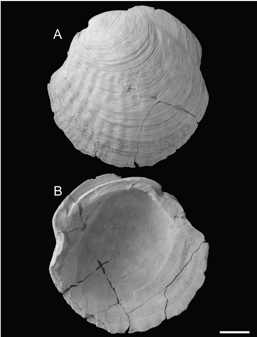
Fig. 2. Holotype of Bulcanites obtusiplicatus sp. nov., MGB MF0002, from a riverbed of Bayabas river, barangay Banaban, Angat municipality in Bulacan province. A, Exterior of left valve; B, interior of the same valve. Scale bar: 20 mm.
