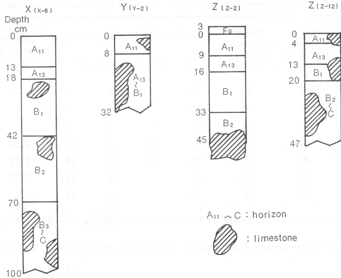
Fig. 6. Diagrammatic profiles of the soil investigated.
