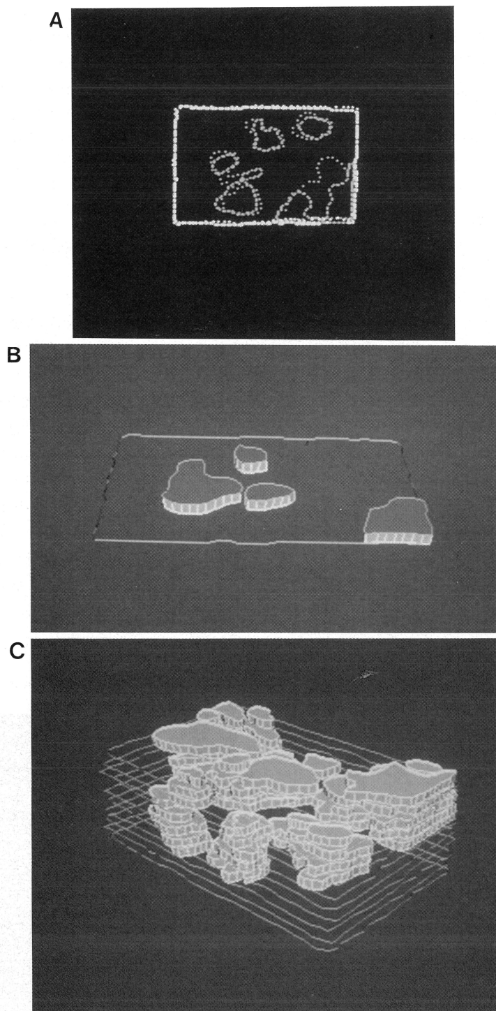
Fig. 4. Voids of soils restructured in three-dimensions by using the three-dimensional construction software with a personal computer.
