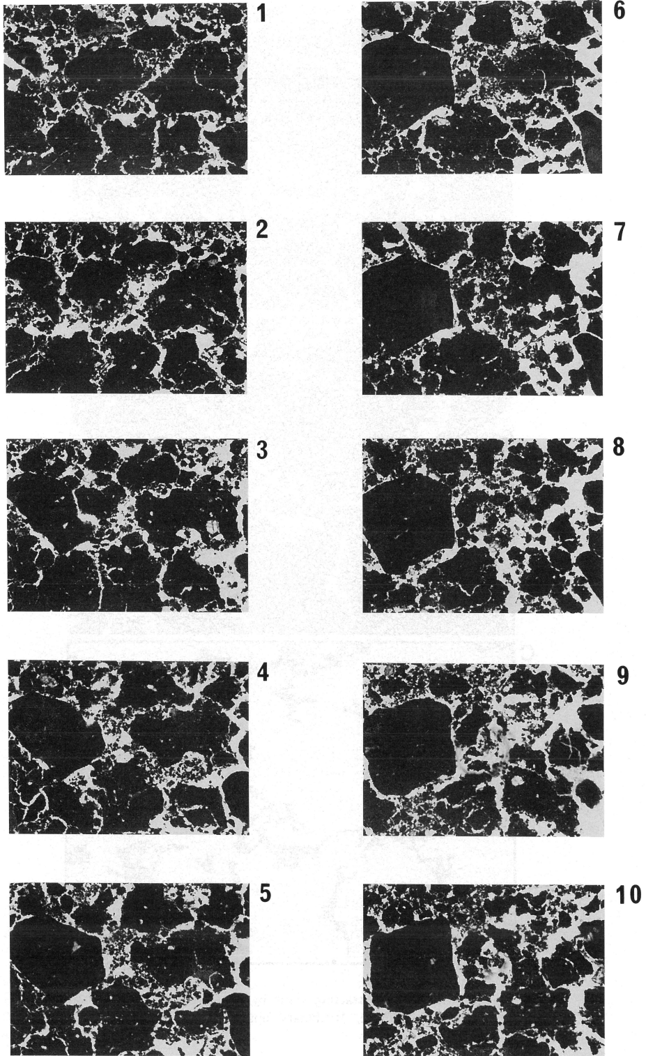
Fig. 2. Consecutive soil thin sections cut out with slicing-machine. (wide length 35 mm)
