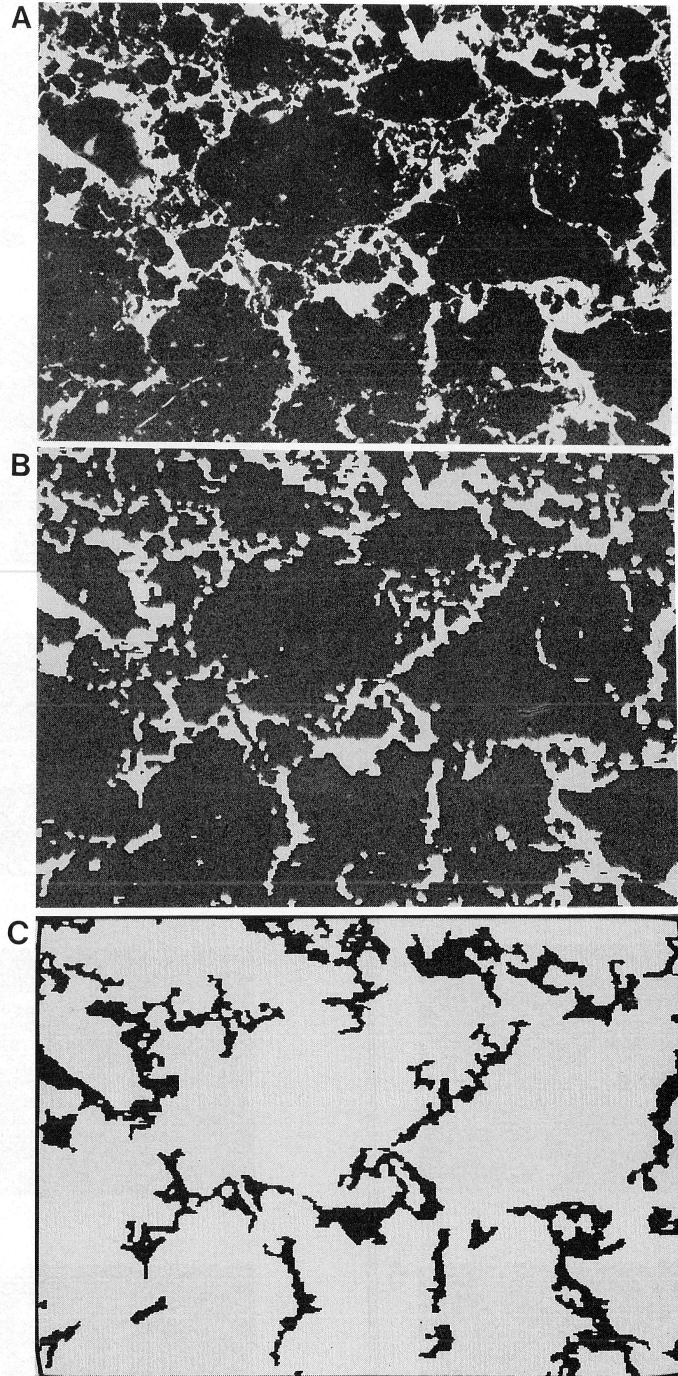
Fig. 3. Method of extracting voids by image analysis. A: original image, B: binary image, C: reversal binary image.
