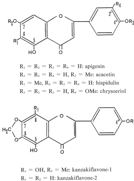
Fig. 2. Chemical structures of flavones isolated from Iris species.
