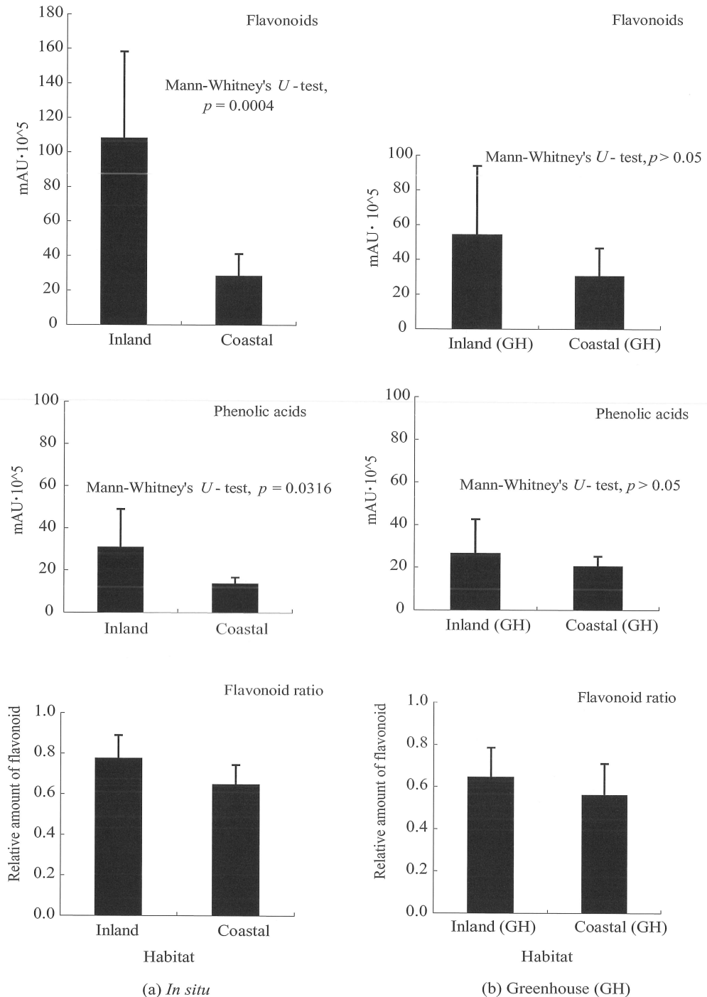
Fig. 3. Amount of the major phenolic compounds in leaves of Adenophora triphylla var. japonica in August 2004. Data of plants growing in the field (a) and in the greenhouse (b) were shown. Vertical axes are the amount of flavonoids, the amount of phenolic acids and flavonoid ratio. All the data of phenolic compounds are shown in Table 2 and Table 3. Error bars indicate the standard deviations. Different letters indicate statistically significant differences at p < 0.05 (Mann-Whitney's U -test).
