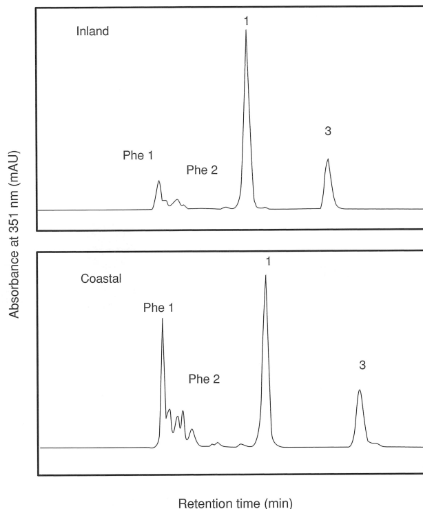
Fig.2. HPLC elution profiles of MeOH extracts from leaves of Adenophora triphylla var. japonica . Profiles of inland and coastal populations are shown. 1 = luteolin 7- O -glucoside, 3 = luteolin 7,4'- O -glucoside, Phe1 and 2 = unknown phenolic acids.
