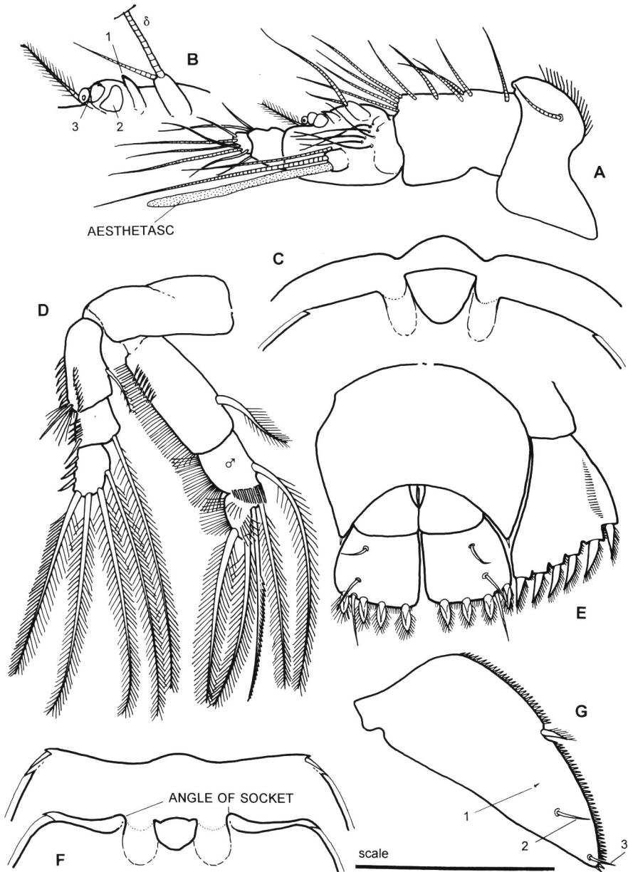
Fig. 2. Clavigofera pacifica . A. Male right antennule, ventral view. B. Detail of coupling denticles. C. Anterior edge of female cephalosome, dorsal and ventral focus. D. Male P2. E. Male urosome, P5 and caudal rami. F. Anterior edge of male cephalosome. G. Female P5, dorsal. Scale bar: A=0.06 mm; C, F=0.19 mm; D=0.082; E=0.1 mm; G=0.135 mm.
