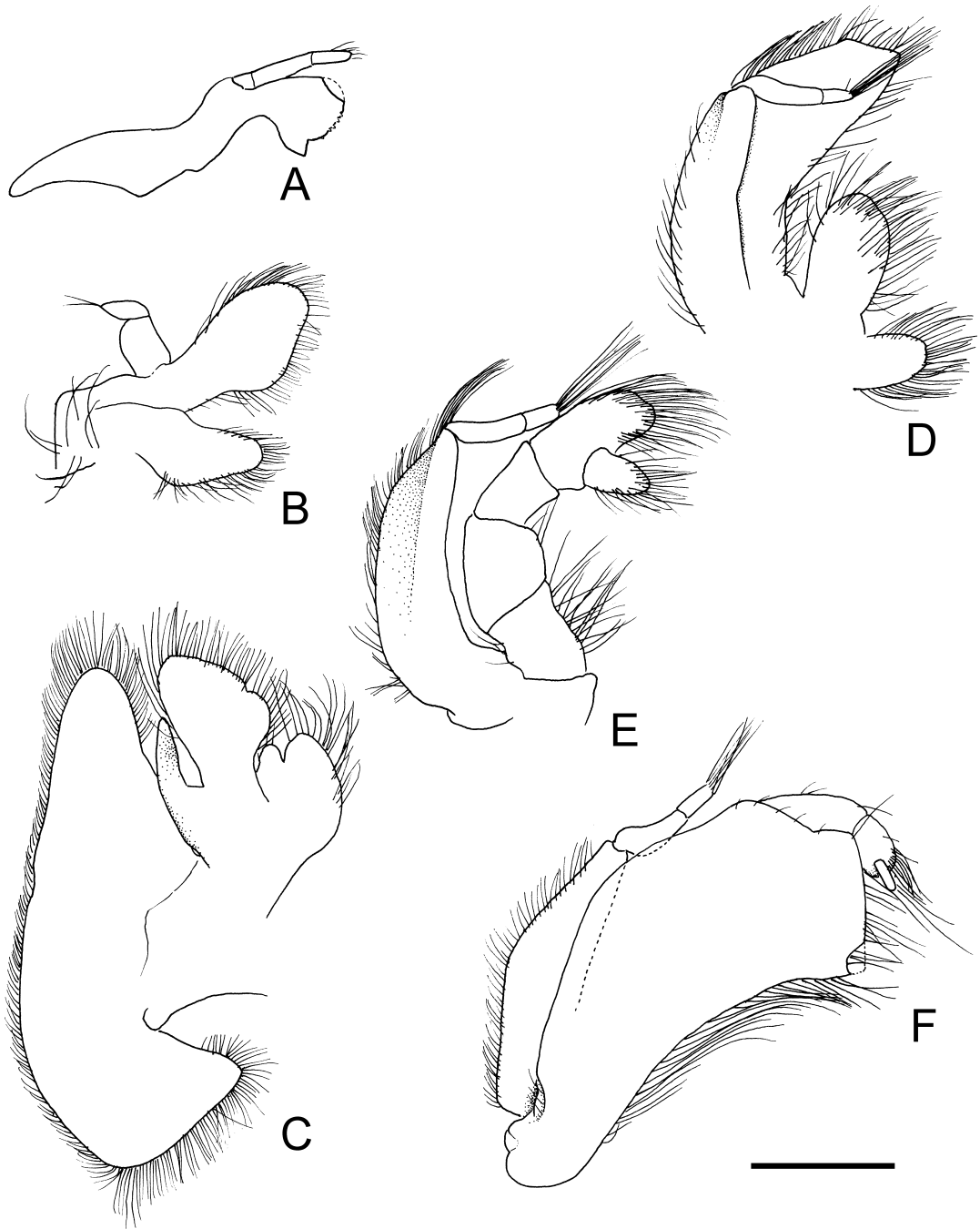
Fig. 3. Abyssotheres aesticola sp. nov., holotype, ovigerous female (NSMT-Cr 19860; cl 11.2×cb 11.1 mm). A, mandible (lacking on mesio-distal corner of incisor process); B, maxillule; C, maxilla; D, first maxilliped; E, second maxilliped; F, third maxilliped (lacking on mesio-proximal angle of merus). Scale 1 mm.
