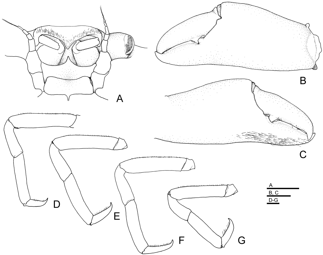
Fig. 2. Abyssotheres aesticola sp. nov., holotype, ovigerous female (NSMT-Cr 19860; cl 11.2×cb 11.1 mm). A, carapace, frontal view; B–C, left chela, outer and inner views, respectively; D–G, left first to fourth walking legs, posterior view. Scales: 1 mm.
