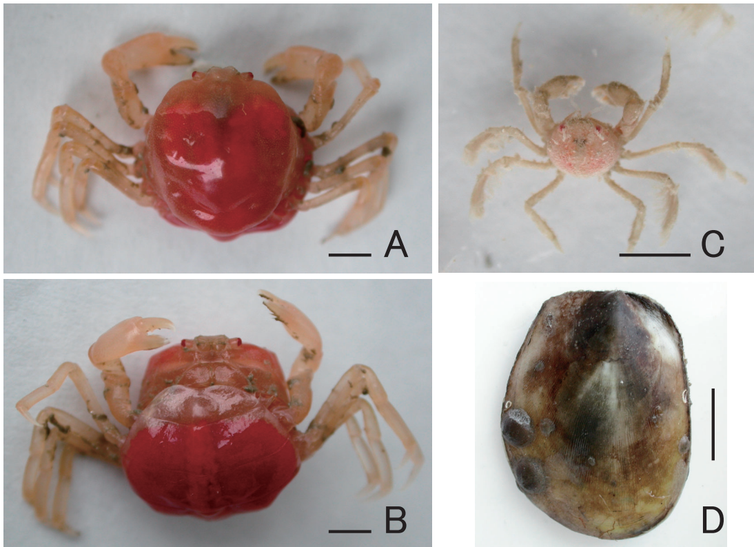
Fig. 1. A–C, Abyssotheres aesticola sp. nov. A–B, holotype, ovigerous female (NSMT-Cr 19860; cl 11.2×cb 11.1 mm), dorsal and ventral views, respectively; C, paratype, male (NSMT-Cr 19861; cl 3.0×cb 2.6 mm), dorsal view. D, Acosta philippinensis (shell height ca 170 mm; id by K. Hasegawa), host of paratype, ovig. female (NSMT-Cr 19862). Scales: 3 mm (A–C), 50 mm (D).
